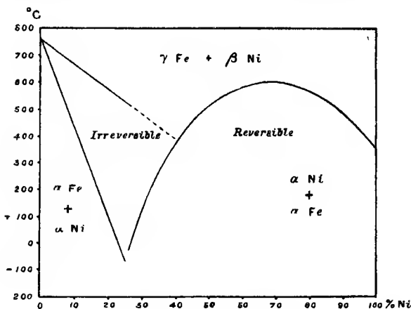
FIG. 108.—Iron-nickel alloys.
